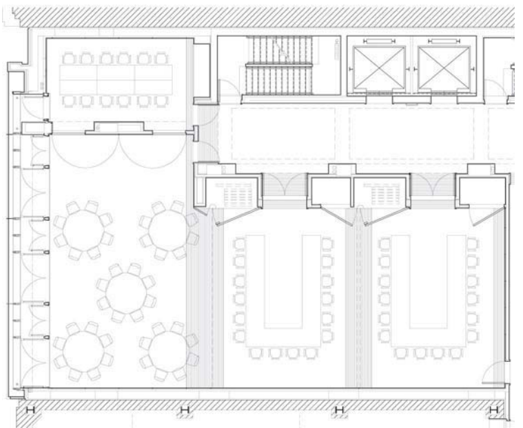
Banquet Room Plan and Section
