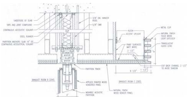
Banquet Room Plan and Section
